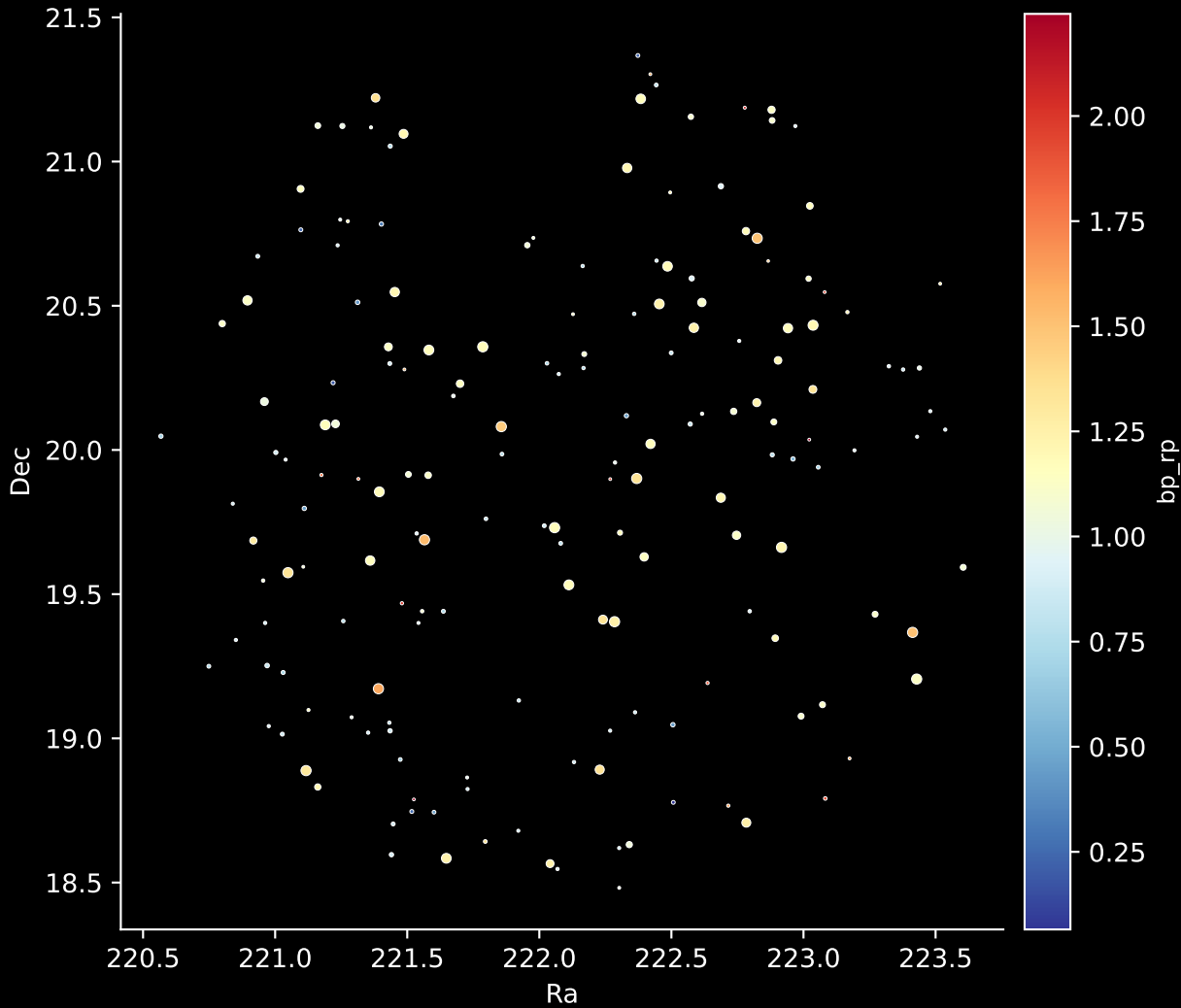
APOGEE DR17 Field: [203+26_MGA] Stars: 177
