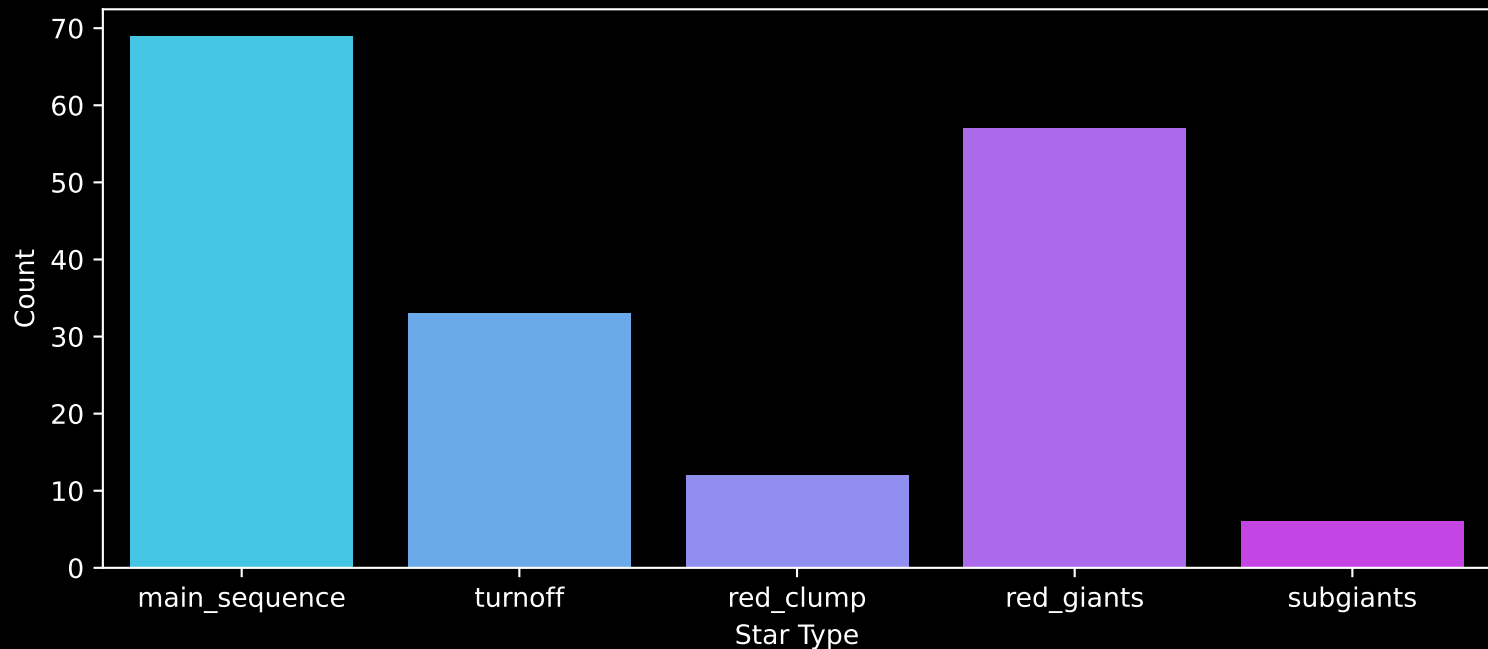
APOGEE DR17 Field: [203+26_MGA] Count plot of Star Type
