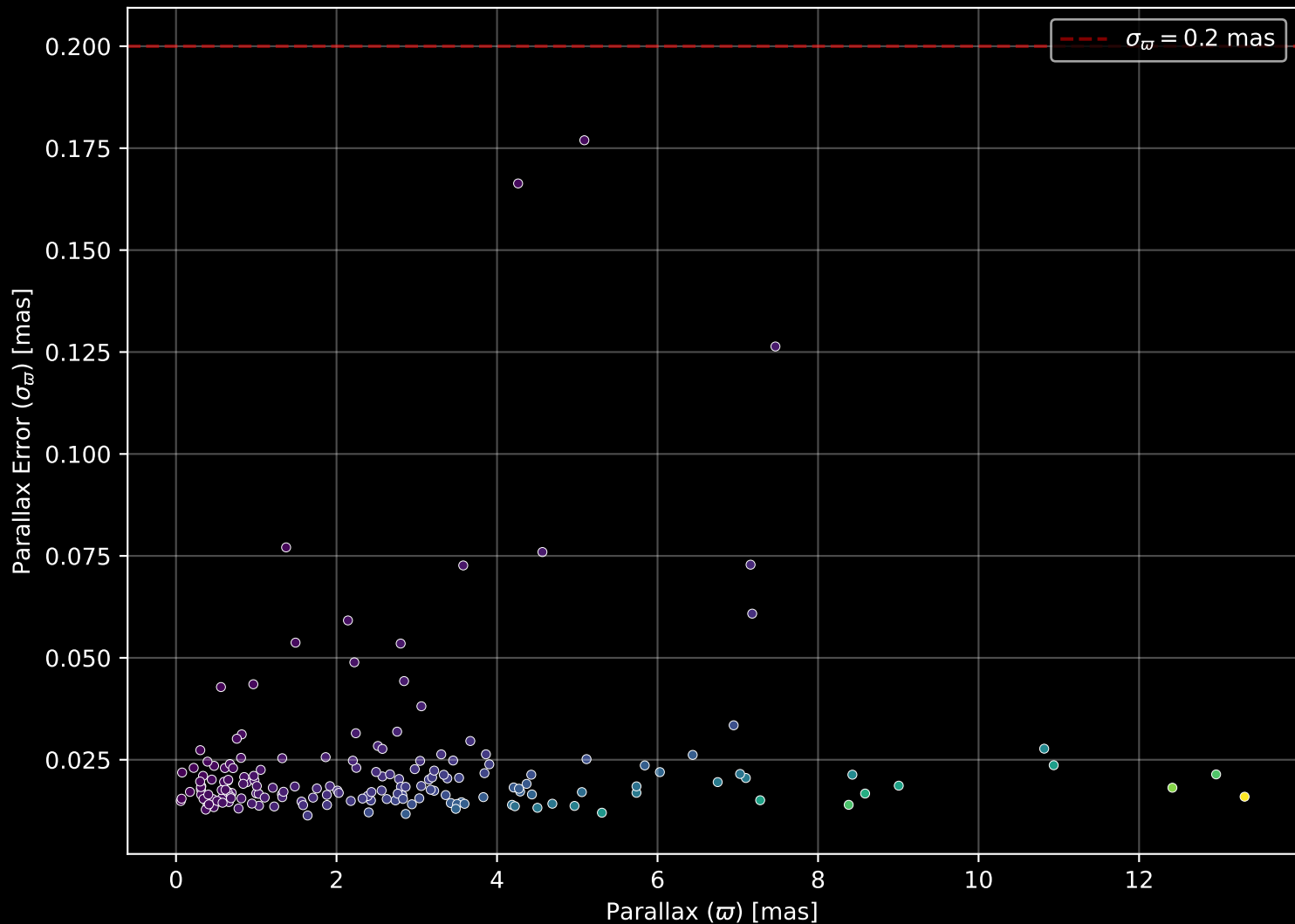
APOGEE DR17 Field: [203+26_MGA] Parallax Quality (n= 177)
