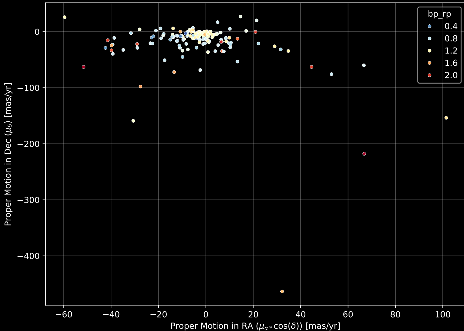
APOGEE DR17 Field: [203+26_MGA] Proper Motion Diagram (n= 177)
