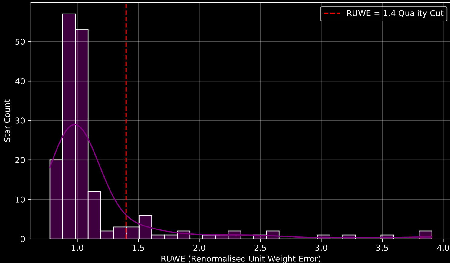
GAPOGEE DR17 Field [203+26_MGA] RUWE Distribution (n= 172)
