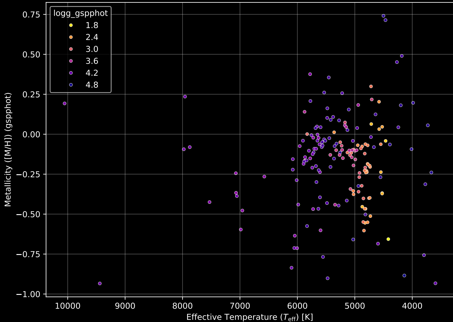
APOGEE DR17 Field: [203+26_MGA] Stellar Population Parameters (n= 177)
